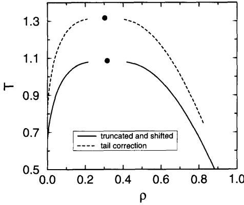
Figure 3.3: Vapor-liquid coexistence curves of various three-dimensional Lennard-Jones fluids: effect of the truncation of the potential on the location of the critical point (large black dots). The upper curve gives the phase envelope for the full Lennard-Jones potential (i.e., a truncated potential with tail correction); the lower curve gives the envelope for the potential that is used in most Molecular Dynamics simulations (truncated and shifted potential with r_c = 2.5\sigma ), data from [53].
