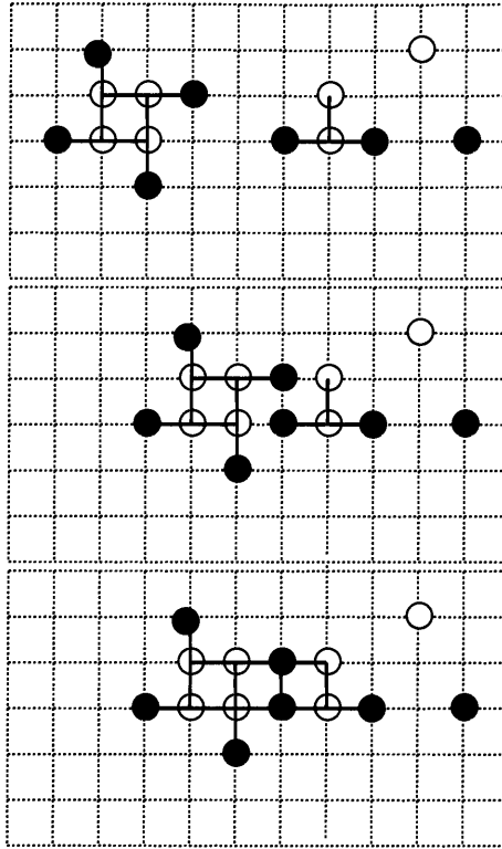
Figure 14.4: Violation of detailed balance in a cluster move; the top figure shows the four clusters in the system; in the middle figure one of the clusters is given a random displacement, which brings this cluster into contact with another cluster; and the bottom figure shows that new configuration has only three clusters if the moves have been accepted.
