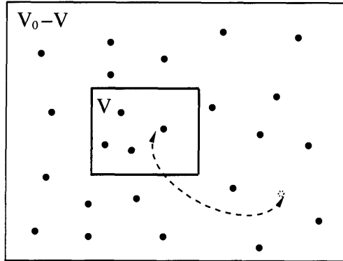
Figure 5.7: Ideal gas ( M - N particles, volume V_0 - V ) can exchange particles with a N -particle system (volume V ).
