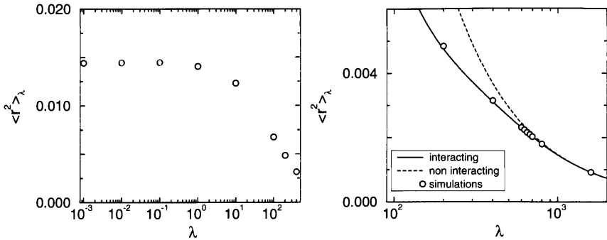
Figure 10.3: The mean-squared displacement \langle r^2 \rangle_\lambda as a function of the coupling parameter \lambda for a hard-sphere (fcc) solid of 54 particles (6 layers of 3 \times 3 \times 3 close-packed atoms at a density \rho = 1.04 ). The figure on the left shows the simulation results for low values of \lambda , the figure on the right for high values. The solid line takes into account nearest-neighbor interactions (10.3.31); the dashed line assumes a noninteracting Einstein crystal (10.3.30). The open symbols are the simulation results.
