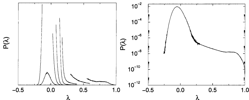
Figure 16.7: (left) P(\lambda, i, t = 3.0) for all slices i . (right) P(\lambda, t = 3.0) when all slices i are combined. The units on the y axis are such that \int_{-\infty}^1 d\lambda P(\lambda, t) = 1 .
